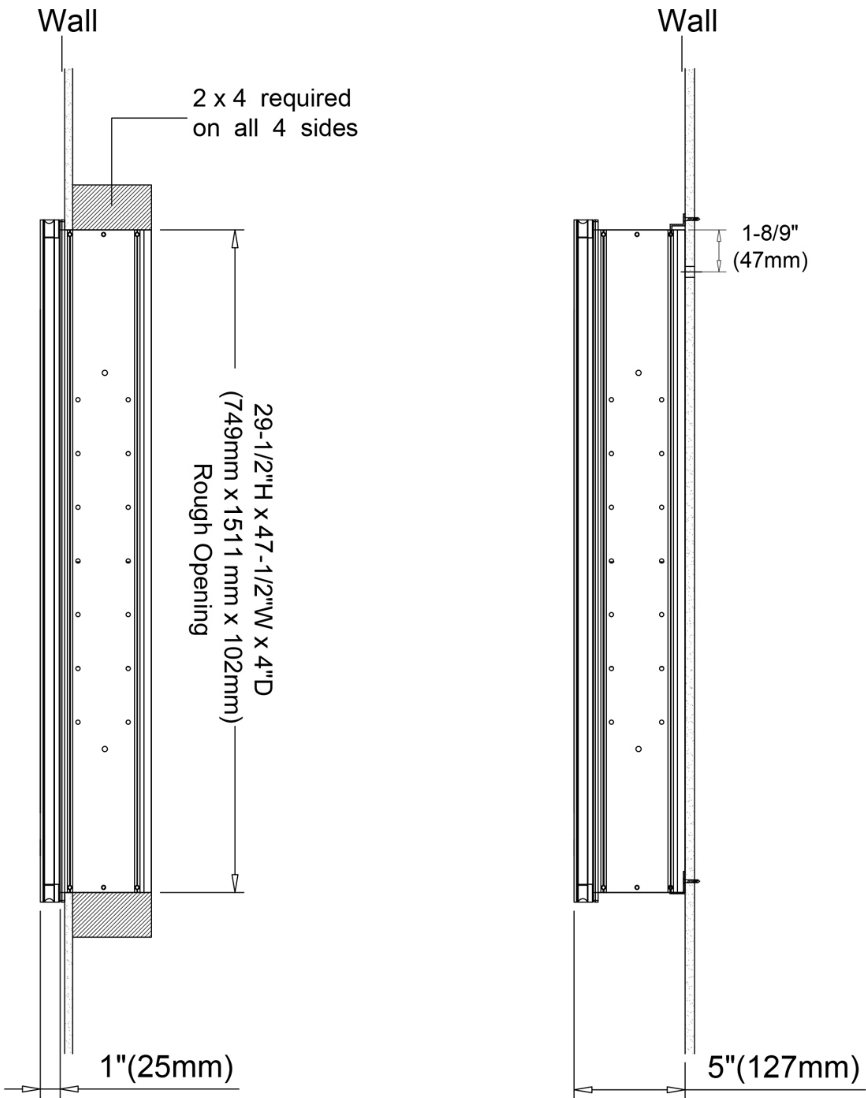
Recessed Mount
