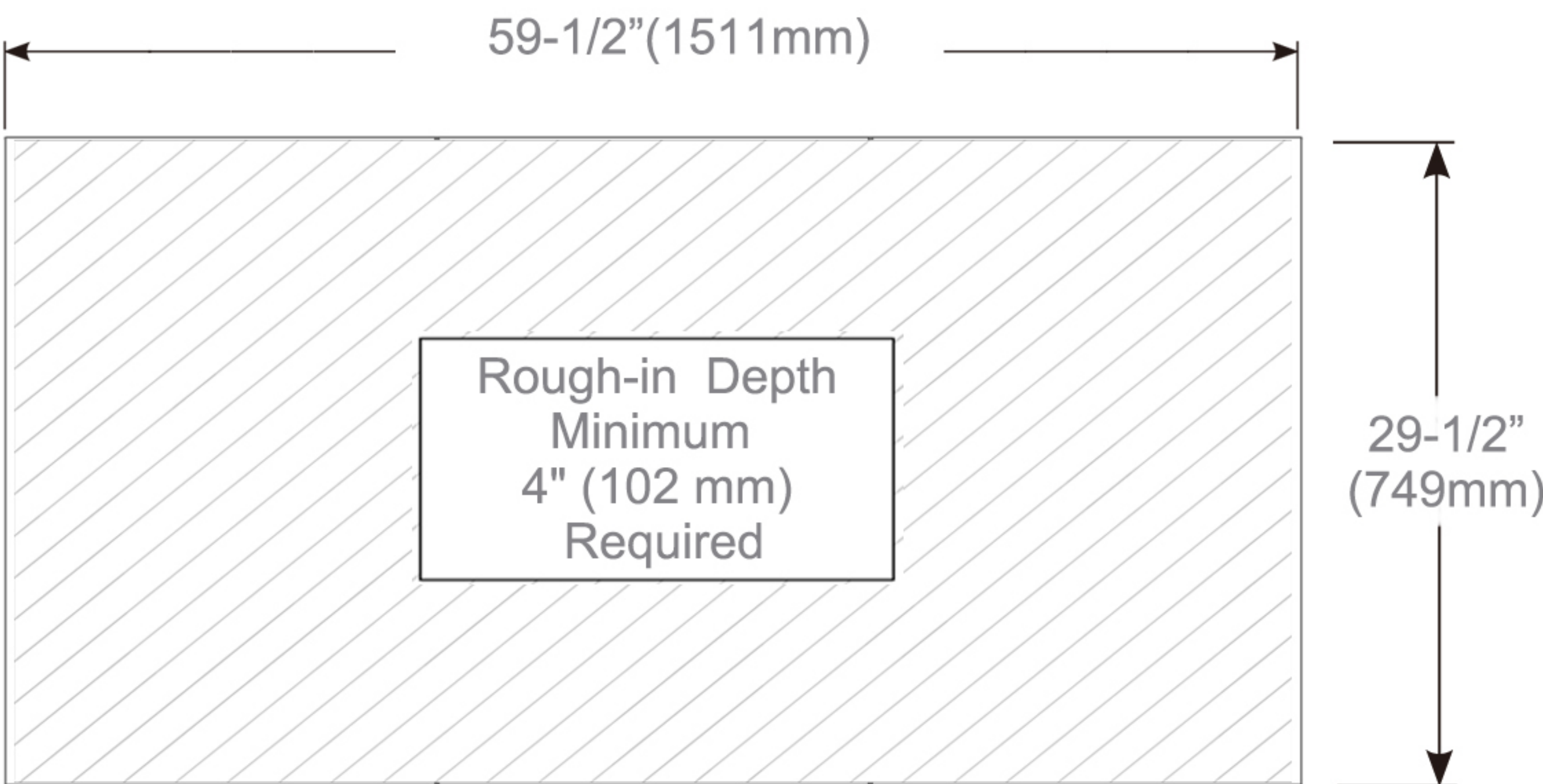
Rough-in Dimensions
