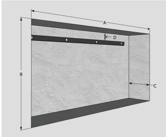
Recessed Opening Sized for Quadra Fireplace
