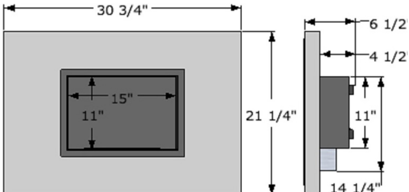
Quadra Fireplace Dimensions
