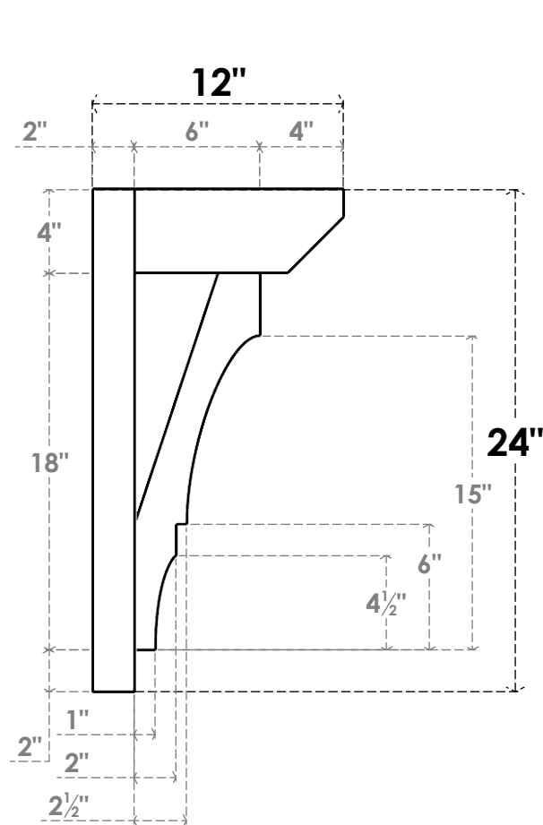
SIDE PROFILE
