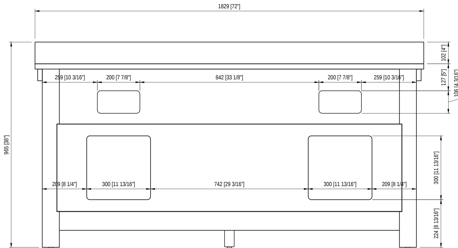
BACK VIEW
