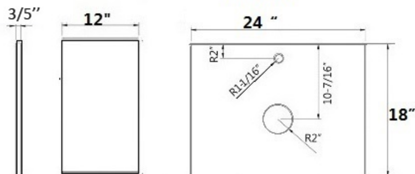
SIDE CABINET TOP
