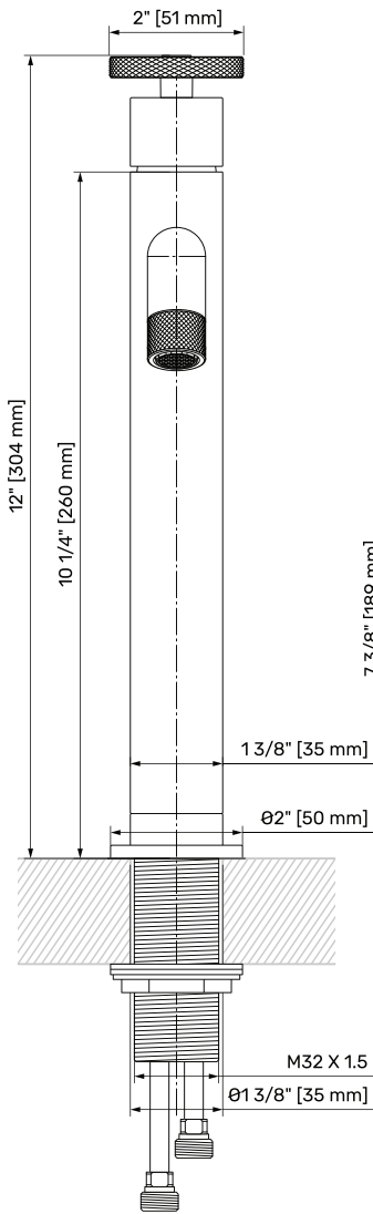
FRONT VIEW / VISTA FRONTAL / VUE DE FACE
