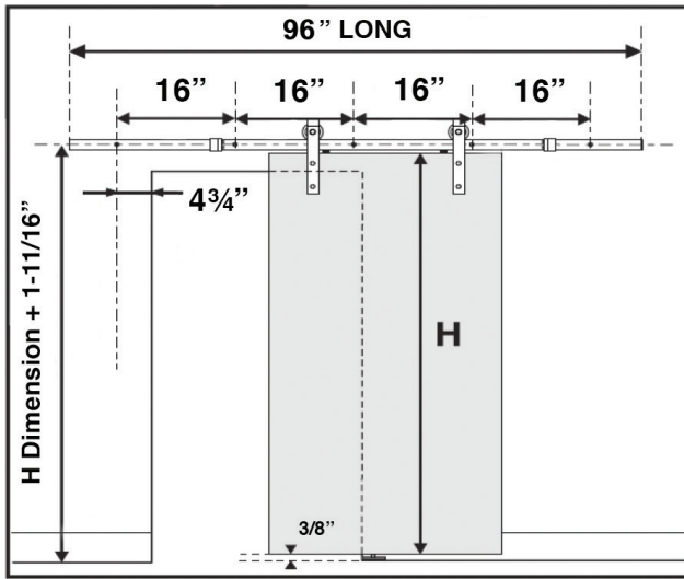
Suggested wall bracket spacing.
