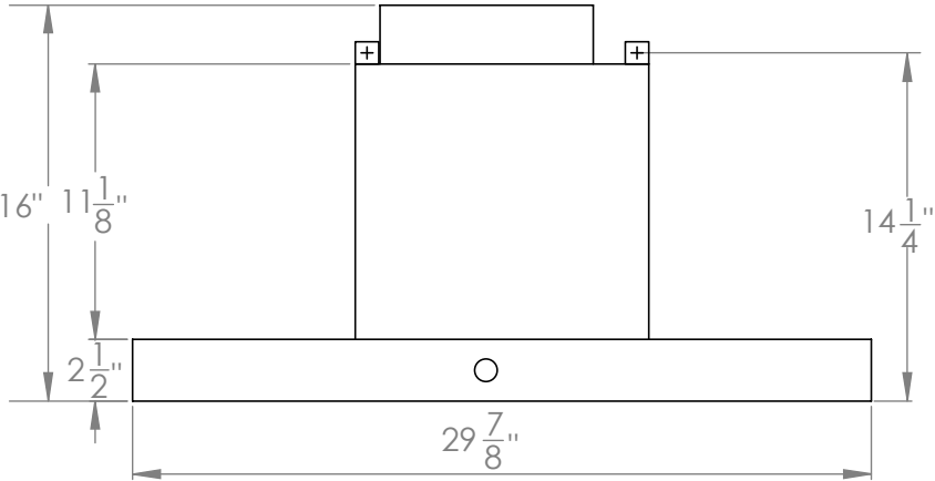
FRONT
