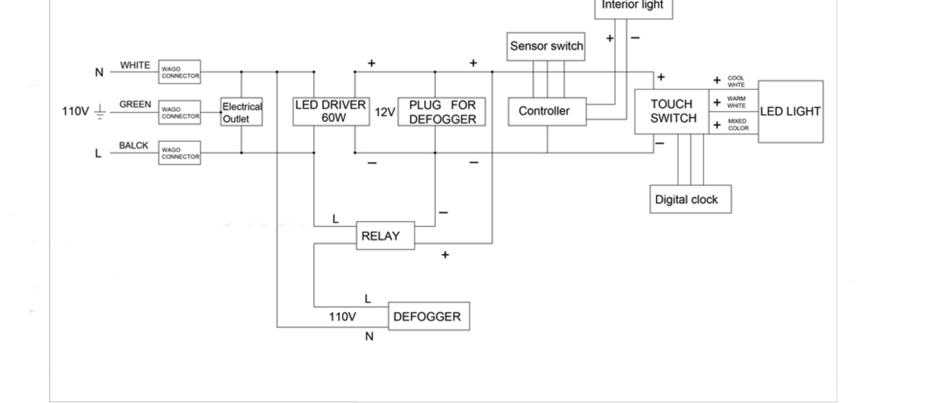
Circuit Diagram
