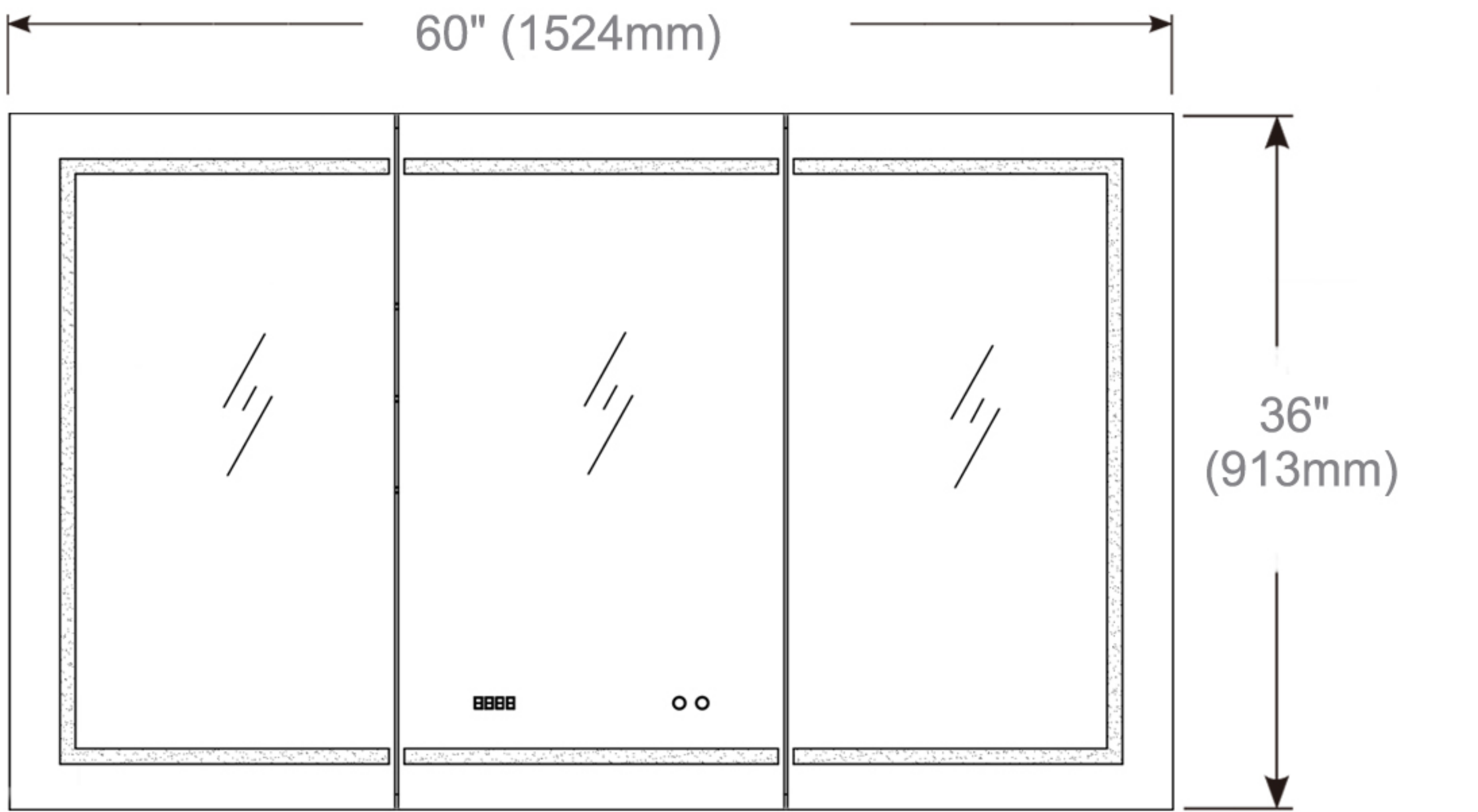
Cabinet Dimensions
