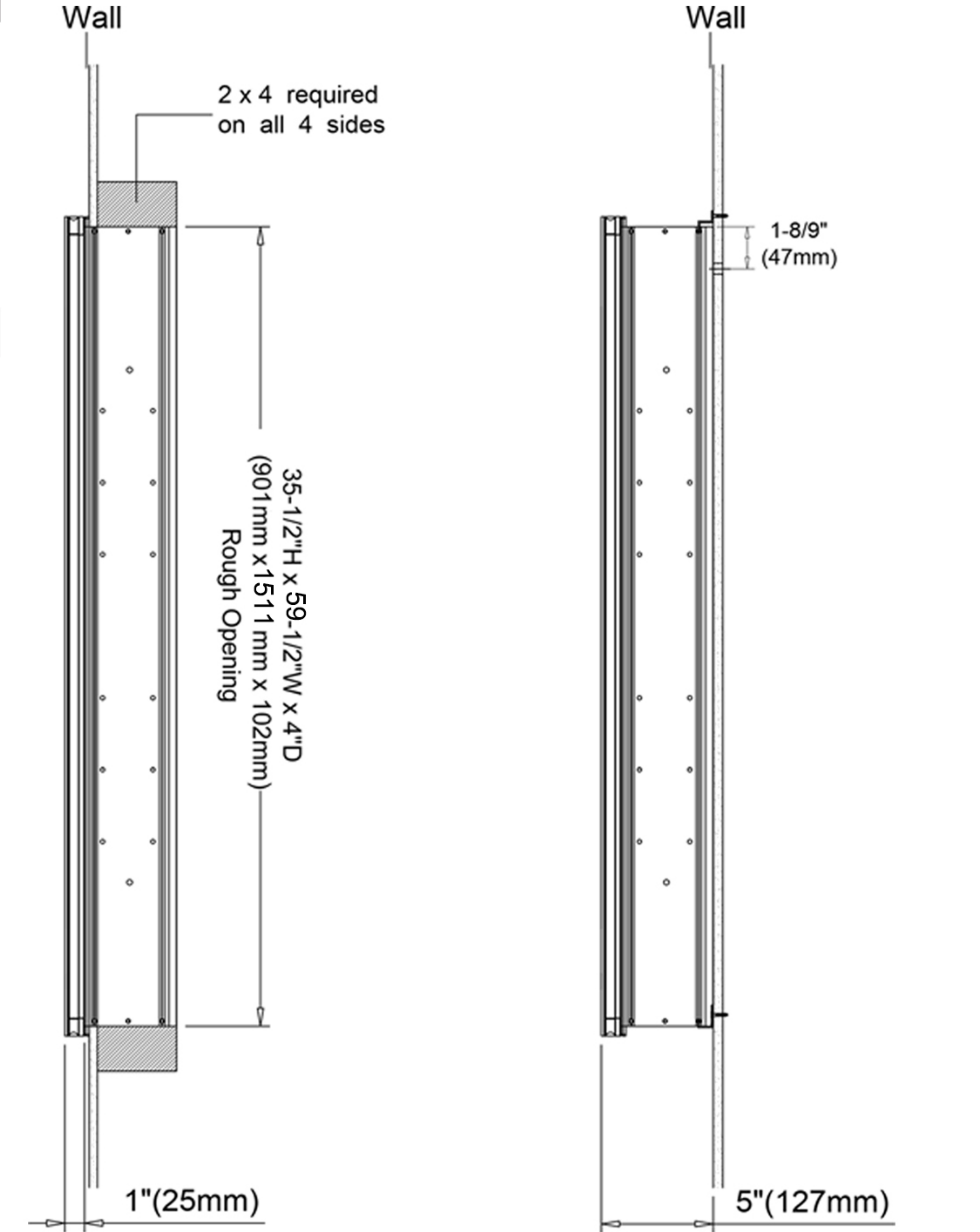
Recessed Mount
