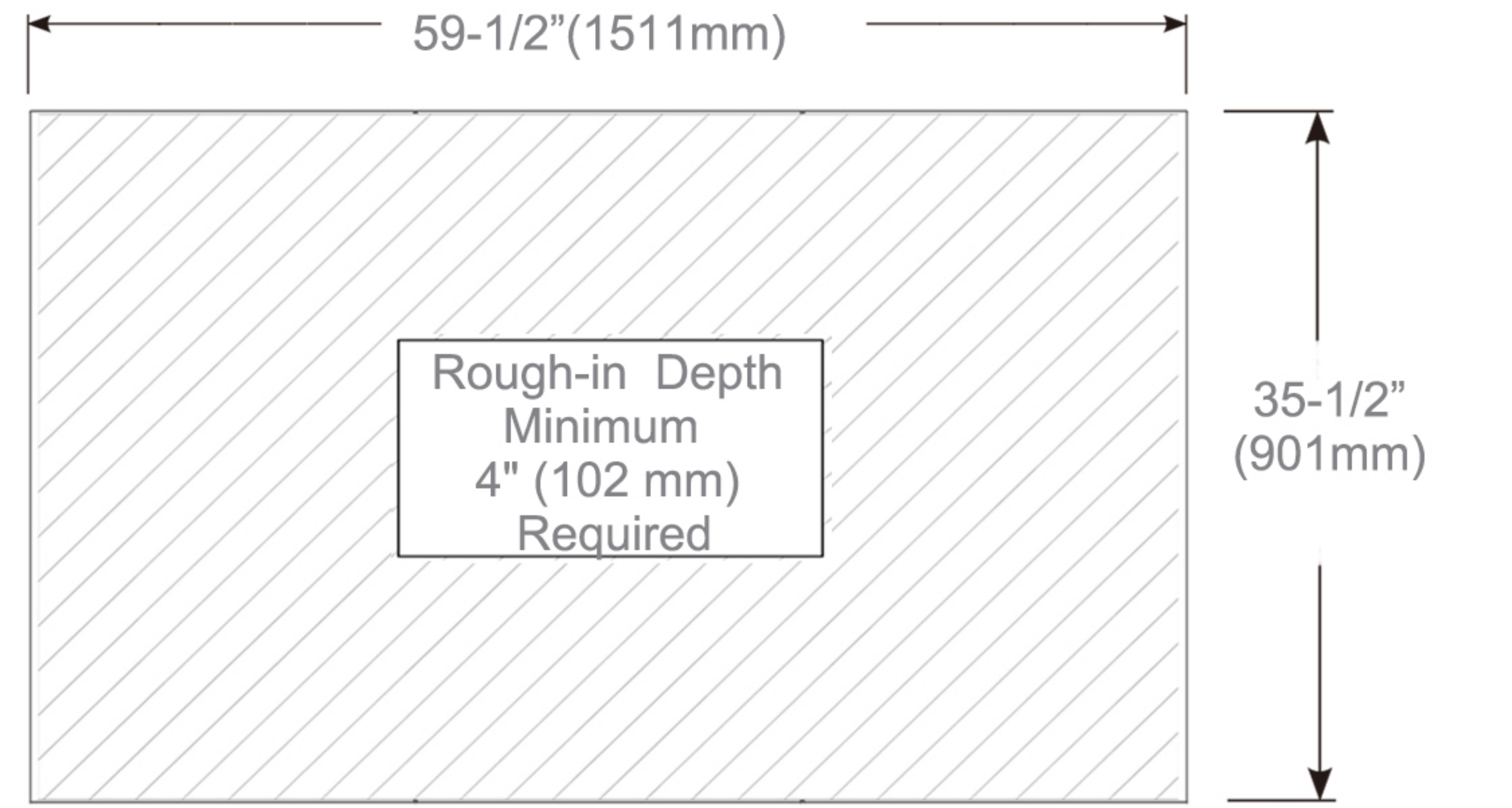
Rough-in Dimensions
