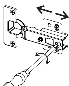
Depth adjustment
