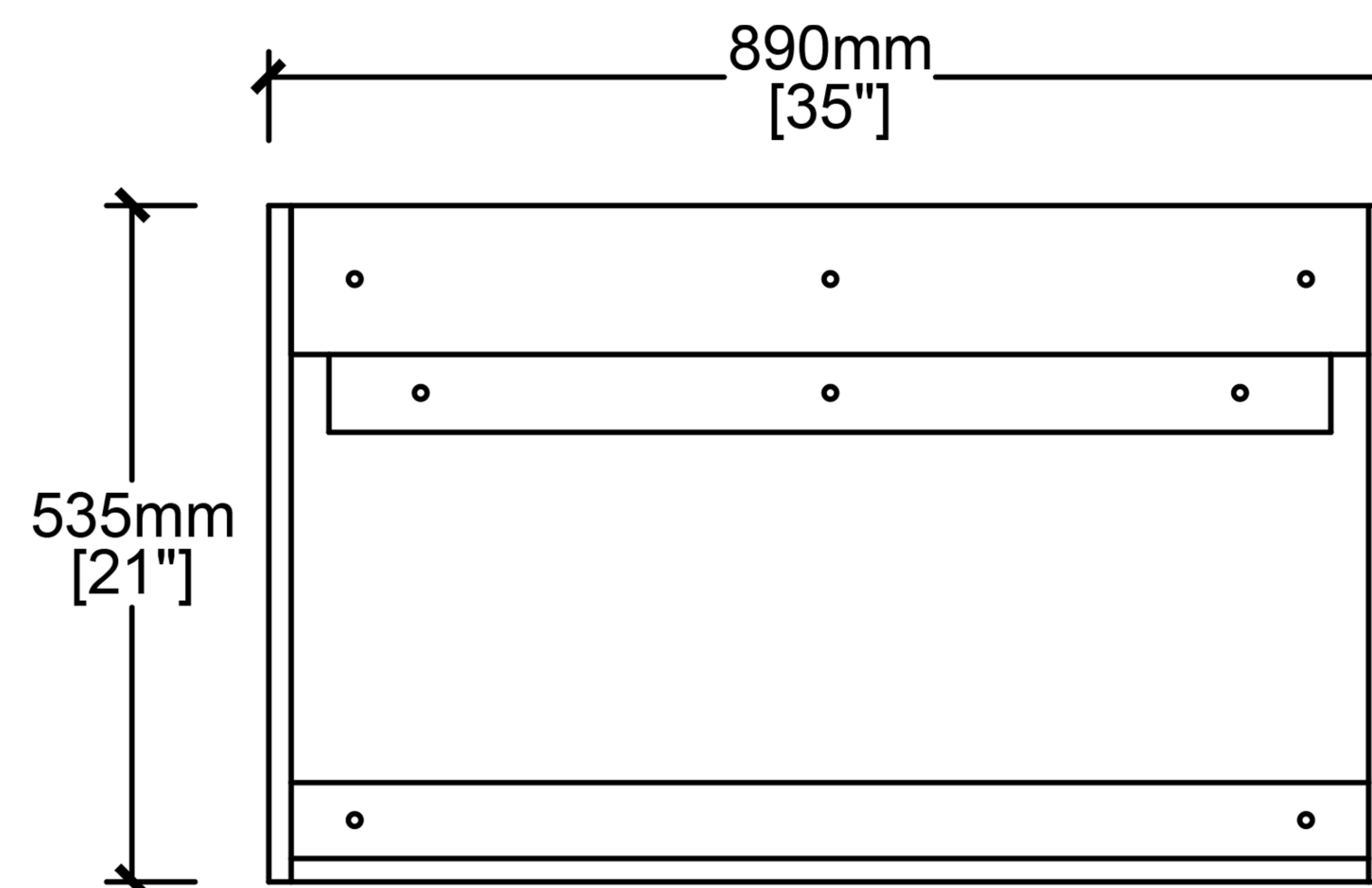
Rear View
