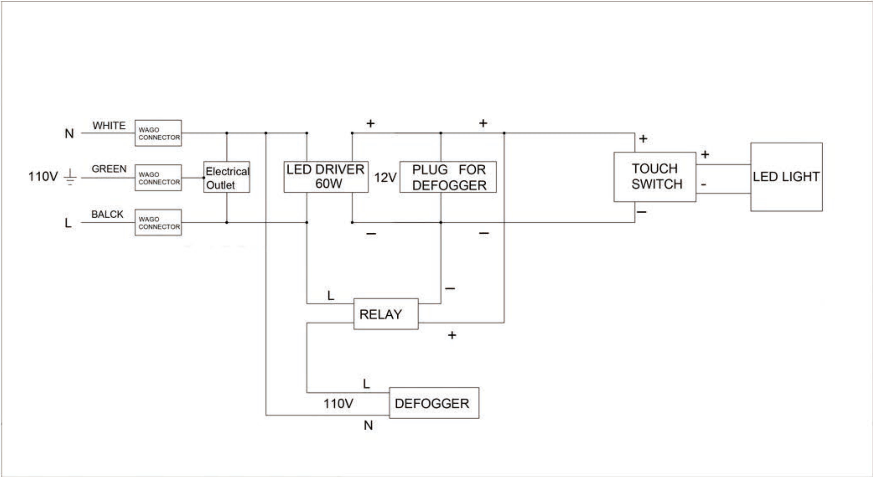
Circuit Diagram
