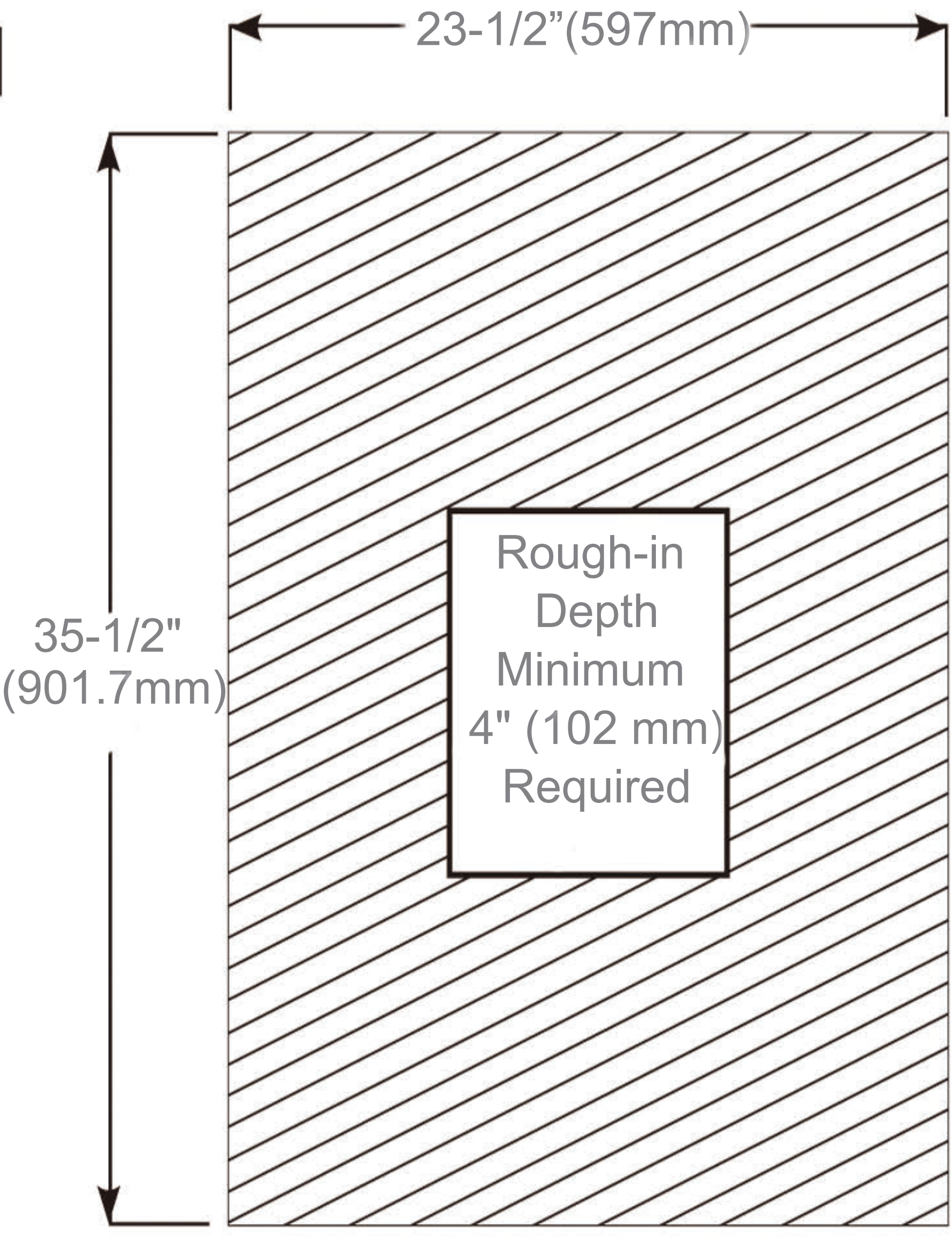
Rough-in Dimensions
