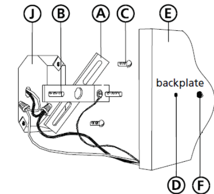
Drawing 3 – Fixture Assembly
