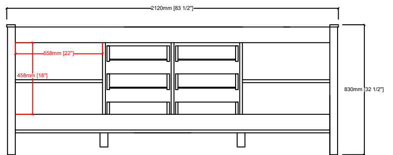
BACK VIEW
