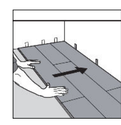
9 After 2-3 rows. Adjust the distance to the front wall by leaving an expansion gap of 1/4". Always ensure that the end joints are staggered at least 8", both when in the same row as when from one row to the next one.
