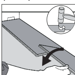
1 After thoroughly cleaning the subfloor, install the 6-mil poly underlayment Polythen you should begin laying in the left-hand corner. Place the floorboard 1/4" from the left wall. Use spacers between the wall and the floorboard.
