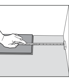
4 At the end of the first row, leave an expansion gap of 1/4" to the wall and measure the length of the last plank to fit.
