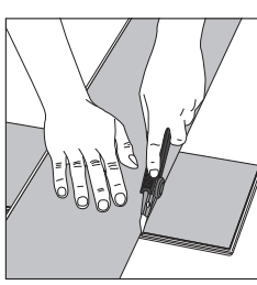
5 To cut the plank, use a simple utility knife and ruler, and with the top side facing up, cut heavily and several times on the same axis. The knife will not go through the surface but make a deep cut. You can then lift one half of the plank using your other hand to hold down the second placing it very close to the cut. The plank will split naturally.
