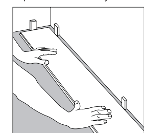
1 After thoroughly cleaning the subfloor, install the 6-mil poly underlayment Polythen you should begin laying in the left-hand corner. Place the floorboard 1/4" from the left wall. Use spacers between the wall and the floorboard.
