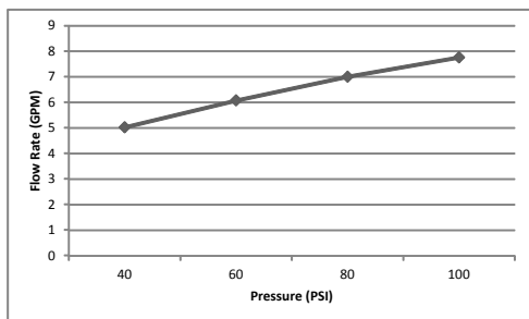
P-2304B Flow Rate (GPM) Vs Pressure (PSI) For Tub Port*
