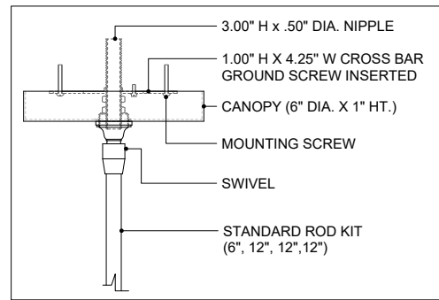
CANOPY DETAIL
