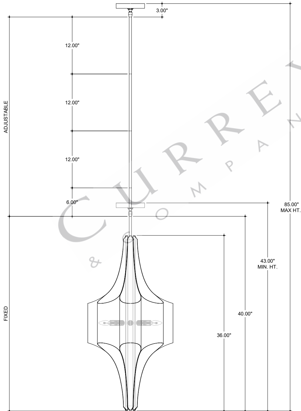
FRONT VIEW
