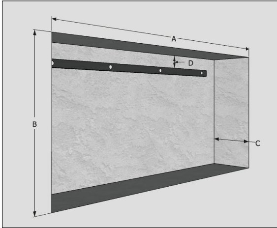
Recessed Opening Sized for Accalia Fireplace
