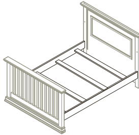
Torino Full-Size Bed Rails – 1216 W:55 x D:75 x H:45.25
